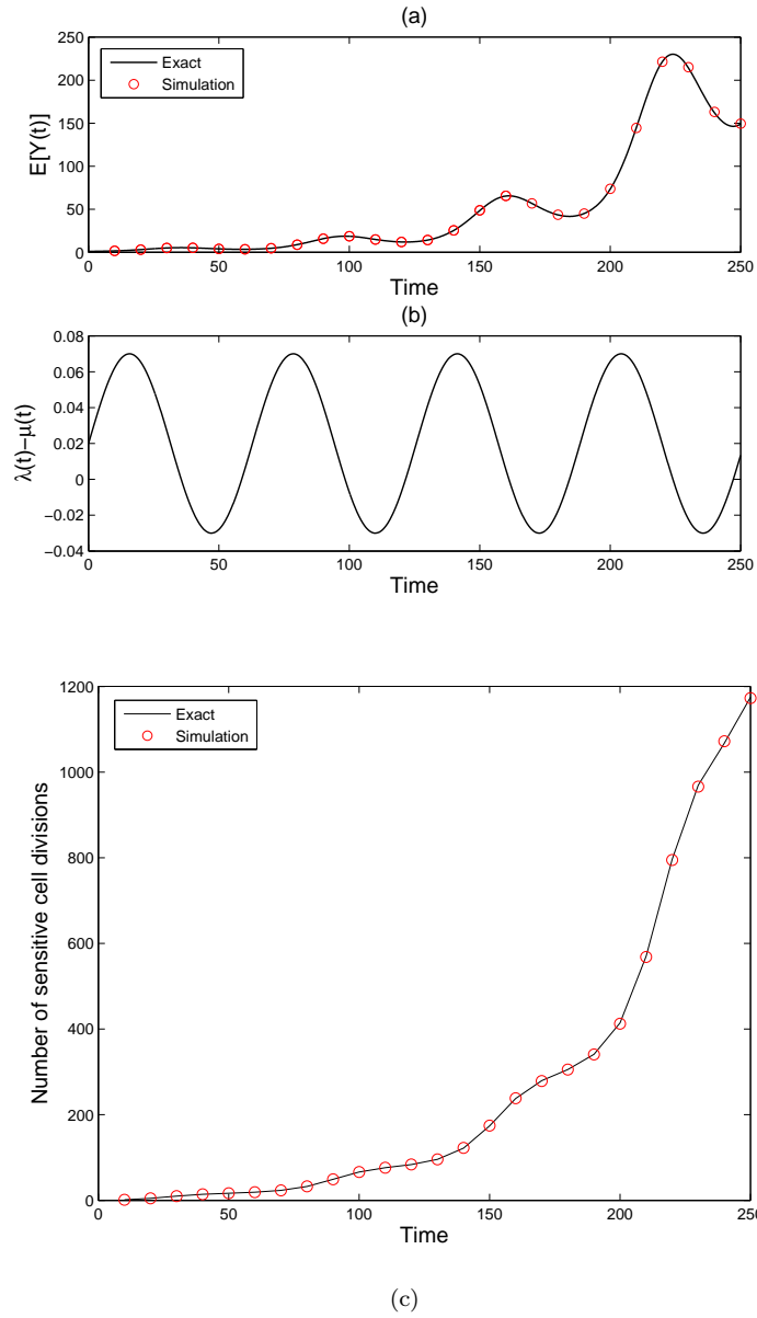
Figure 1: A single-type non-homogeneous birth-death process. (a): Simulation (red circles) and theoretical (black line) mean of the single-type birth and death process Z(t) with birth rate \lambda(t) = 0.05 \sin(0.1t) + .1 , death rate \mu(t) = .08 and initial population size M = 1 . (b) We plot the net growth minus death rate \lambda(t) - \mu(t) as a function of time. (c) We show the number of sensitive cell divisions for the process Z(t) with birth rate \lambda(t) = 0.05 \sin(0.1t) + .1 , death rate \mu(t) = .08 and initial population size M = 1 . Simulation (red circles) and theory (black line) are shown.
