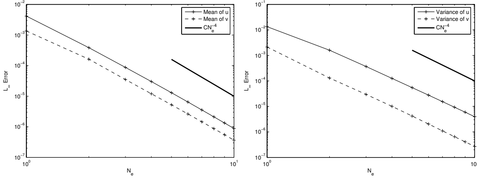
Fig. 10. Kovasznay flow problem: h -convergence rate for \xi \sim B(-1,1) . Left: mean; Right: variance.
