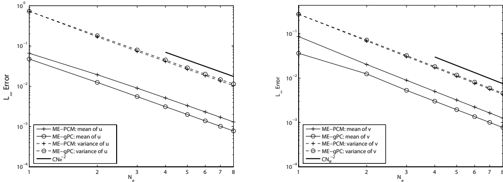
Fig. 11. Kovasznay flow problem: h -convergence rate for \xi \sim B(0,0) . Left: x -velocity; Right: y -velocity.
