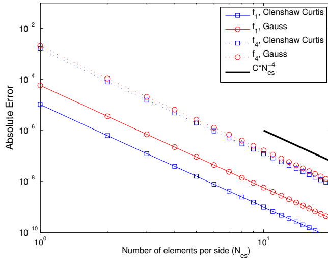
Fig. 1. h -convergence of Gauss and Clenshaw-Curtis sparse grid integration of smooth functions f_1 and f_4 from the GENZ test suite. Solid lines indicate f_1 errors while dotted lines indicate f_4 errors. Square markers: Clenshaw-Curtis points, circle markers: Gauss points.
