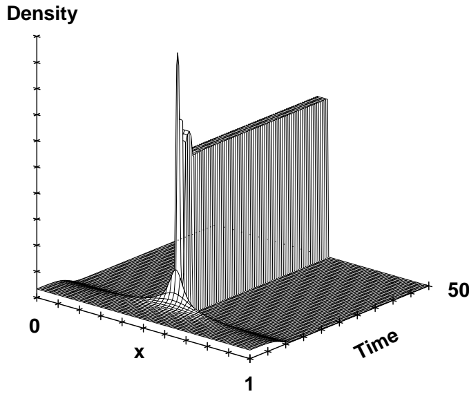
FIG. 13. The evolution of p for the solution of (100) with \gamma_r = \nu = 0 and \mu = 1 . The initial data are as in Figure 6. p_{peak} = 30.15 , p_{min}(50) = 1.82 \times 10^{-4} , p_{max}(50) = 18.18 .
