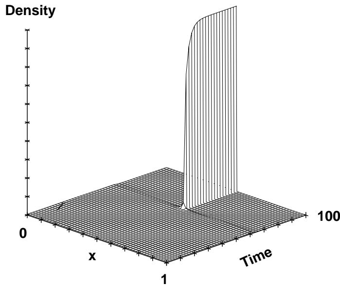
FIG. 14. The evolution of p for the solution of (100) with \nu = 1 \times 10^{-5} and \mu = 1 . The initial data are as in Figure 6 for p , but w is set to 1. \times 10^{-3} everywhere. p_{min}(100) = 1.97 \times 10^{-3} , p_{max}(100) = 199.6 .
