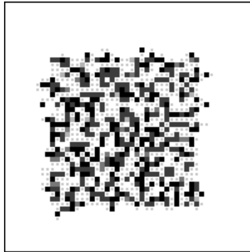
FIG. 3. This figure shows the discrete density distribution for 1000 bacteria after 1000 jumps, using Davis's movement rules with a_1 = 1 and a_j = 1 + 1 + \sum_{k=1}^{j-1} a_k . The bacteria are interacting only via the slime trails. The density of bacteria is coded as follows: black for one bacterium at a grid point, dark gray for two to four bacteria, gray for five and six bacteria, and light gray for seven and more bacteria located at the same grid point. All grid points that have been visited by at least one bacterium are marked by smaller gray squares. All particles are quickly trapped in the sense that they soon oscillate between two points.
