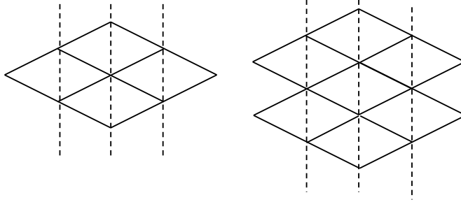
Figure 2: The nodal set and symmetry lines for solutions in Example 4.2.
