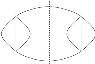
Figure 4: The domain \Omega , and the nodal set and symmetry lines of the solution u from Theorem 4.4.
