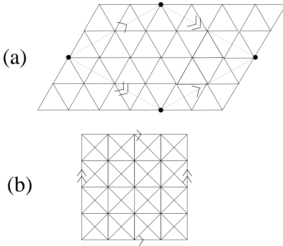
FIGURE 1. Examples of \Delta(G, S) which are 2-tori. In (a), G = \mathfrak{S}_4 and S = (12), (13), (14) (cf. [9, Figure 2]). In (b), G is group of 4 \times 4 unitriangular matrices over \mathbb{F}_2 and S is the subset of unitriangular matrices having one non-zero superdiagonal entry and all other entries above the diagonal zero.
