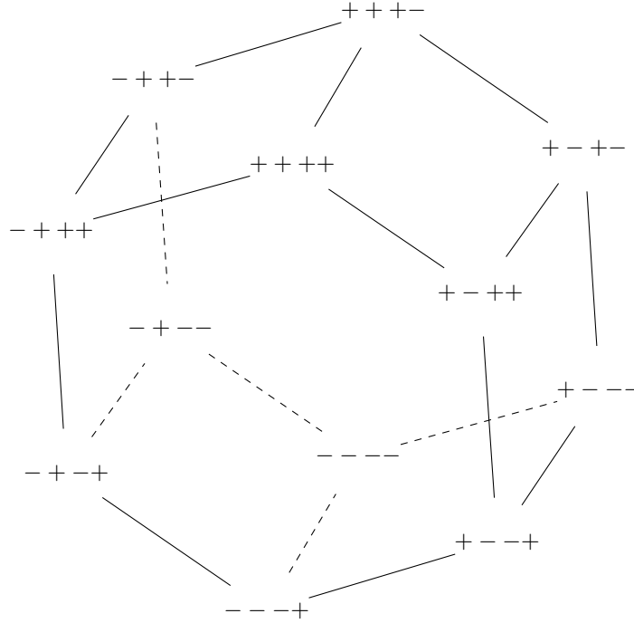
FIGURE 4.1. Zonotopes of Z(\mathcal{A} \sqcup \mathcal{A}') in Example 4.2
