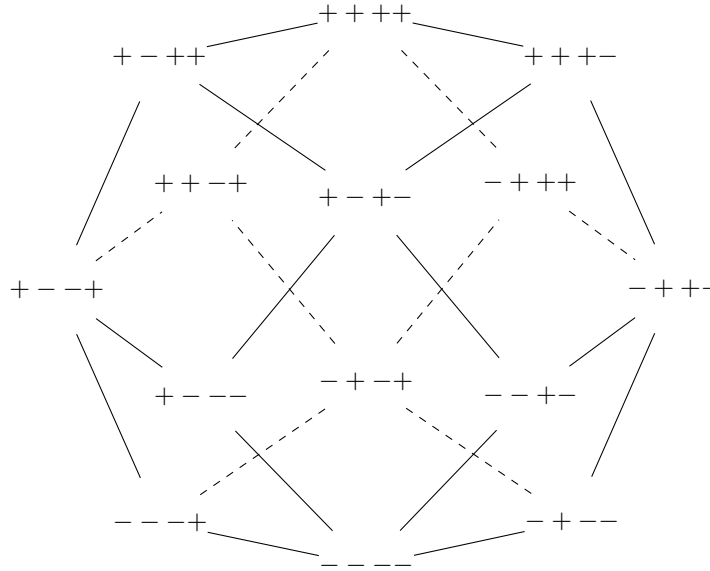
FIGURE A.3. The tiger-tope
