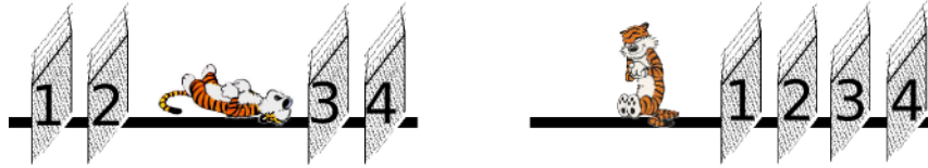
FIGURE A.1. The tiger problem
