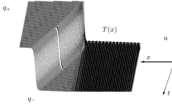
Fig. 2.10. The wedge of an unstable state formed between a small amplitude front of Turing patterns T(x) and a large amplitude front connecting q_+ and q_- .
