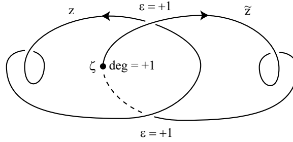
Fig. 2.28. Transverse crossings of planar projections of oriented curves, with associated signs \varepsilon_j = \pm 1 . Note \text{lk}(z, \tilde{z}) = +1 , and \text{twist}(z) = \text{twist}(\tilde{z}) = -1 .
