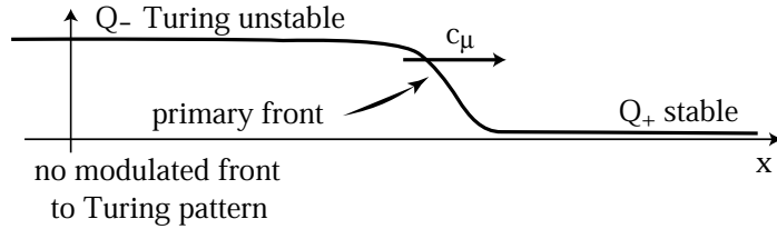
Fig. 2.8. Non-existence of modulated fronts leaving a Turing pattern behind, case II.
