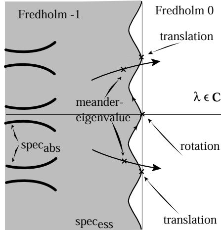
Fig. 2.21. Schematic plot of the meander eigenvalues popping out of the Fredholm index -1 region close to instability.
