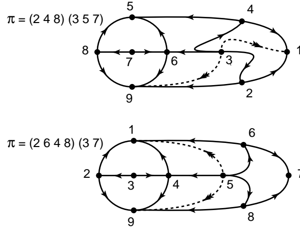
Fig. 2.3. C^0 orbit equivalent Sturm attractors \mathcal{A}_f with nonconjugate permutations \pi_f . Note how the attractors differ in the geometry of the fast unstable manifolds, indicated by double arrows.
