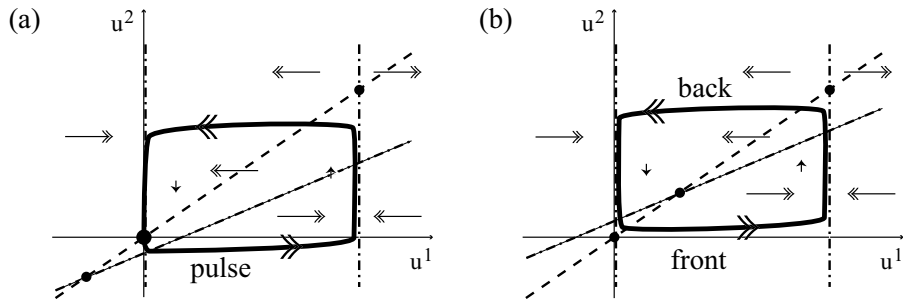
Fig. 2.16. Excitable (a) and oscillatory (b) media; homoclinic pulses and periodic travelling waves for \varepsilon \searrow 0 . Isoclines in absence of diffusion. See also (2.114) for the excitable case (a).
