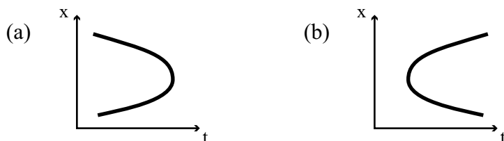
Fig. 2.30. Collision of zeros u(t, x) = 0 for scalar equations: (a) annihilation, (b) creation.
