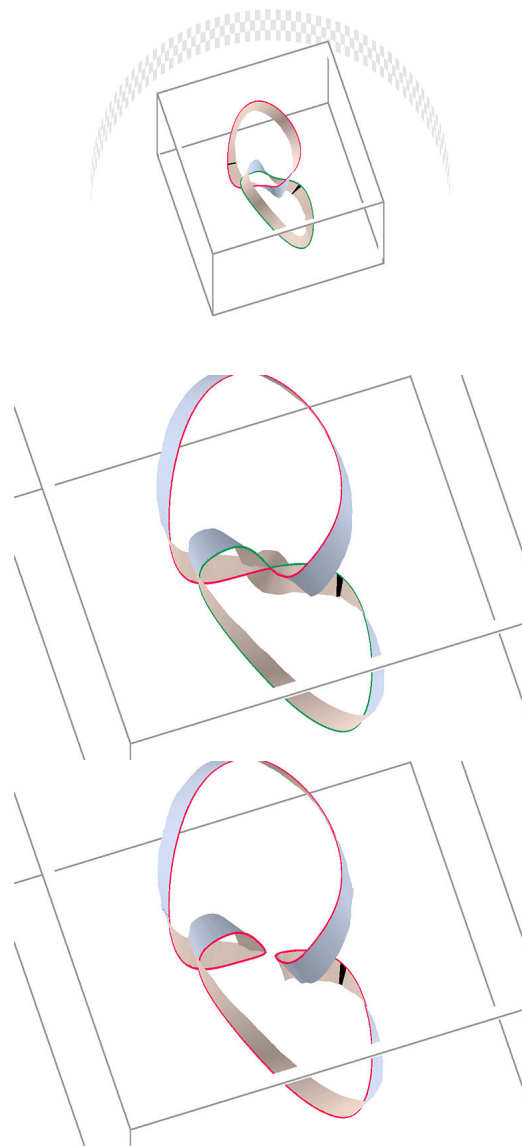
Fig. 2.36. [FiMa00, Fig. 11] Crossover collision of two linked, twisted, circular filaments. See Plate ?? in the Appendix for a version of this figure in colour.
