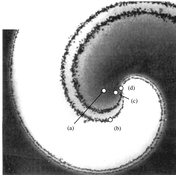
Fig. 2.17. “Tips” of a spiral wave pattern in the BZ reaction: (a) core center, (b) maximum curvature, (c) rotation center, (d) inflection point; courtesy of [MüZy94].
