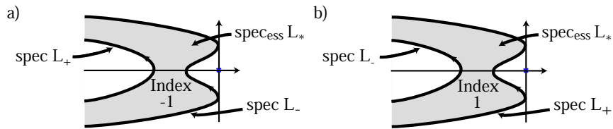
Fig. 2.11. Spectra, Fredholm indices, and oriented critical spectral curves of the linearization about a front, when a Turing instability occurs ahead of the front (a) or behind the front (b).
