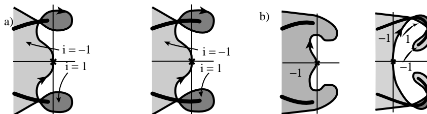
Fig. 2.24. Two scenarios (a), (b) of essential and absolute spectra crossing the axis successively at core-breakup.
