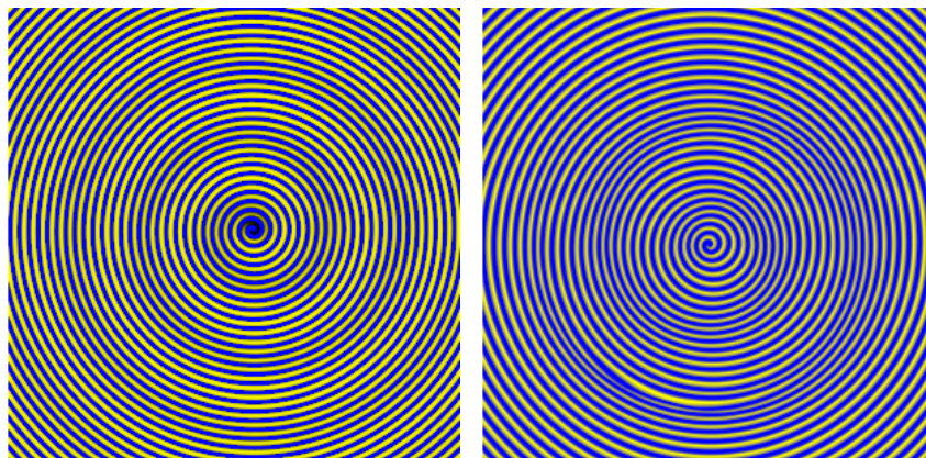
Fig. 2.25. Farfield patterns in case of farfield- and core-breakup. See Plate ?? in the Appendix for a version of this figure in colour.
