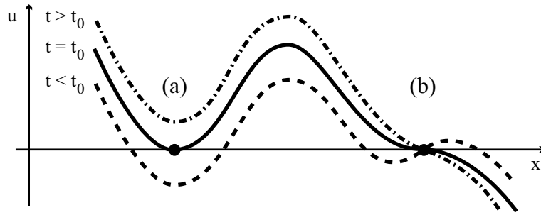
Fig. 2.1. Local dropping of z(w(t, \cdot)) at (a) a double zero, (b) a triple zero of z(w(t_0, \cdot)) .
