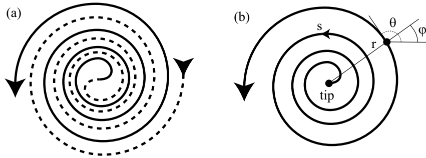
Fig. 2.15. Biasymptotic Archimedean spiral (a), and spiral with spiral tip (b).
