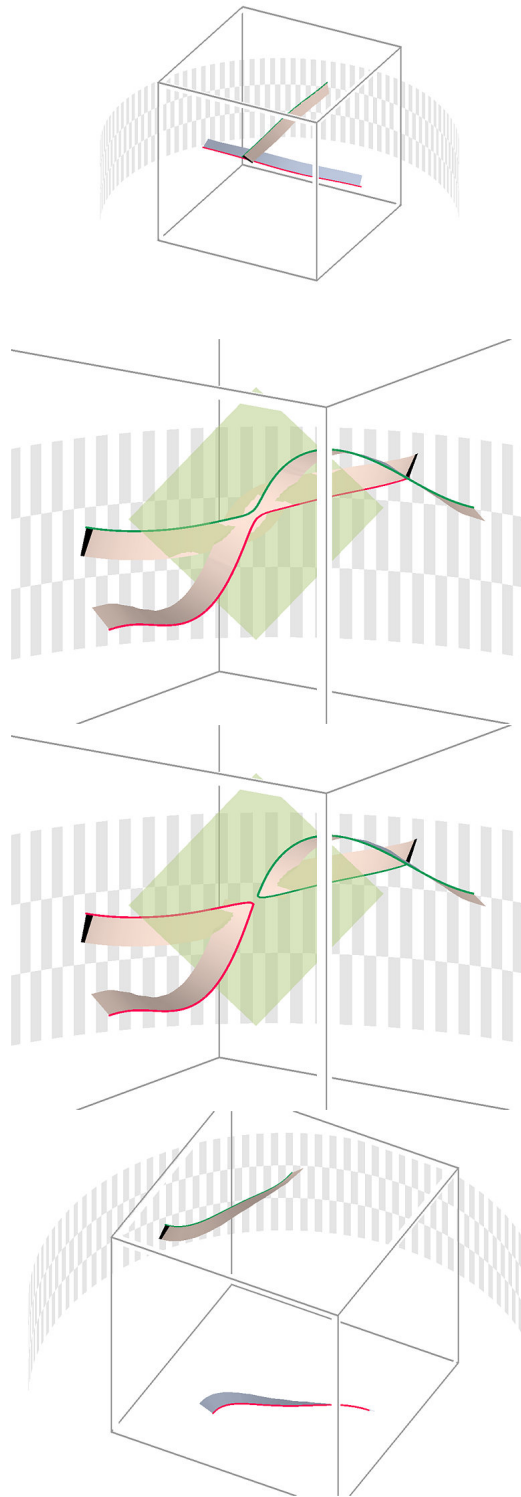
Fig. 2.35. [FiMa00, Fig. 9] Crossover collision of scroll waves including accompanying isochrone bands u_2 = 0 \leq u_1 \leq \delta . See Plate ?? in the Appendix for a version of this figure in colour.
