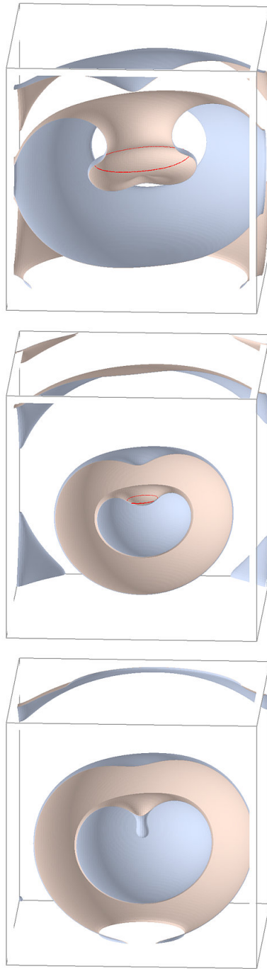
Fig. 2.34. [FiMa00, Fig. 8] Scroll ring annihilation of an untwisted filament. Surfaces u_2 = 0 \leq u_1 shown. See Plate ?? in the Appendix for a version of this figure in colour.
