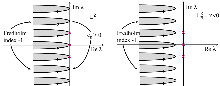
Fig. 2.20. Typical spectrum of the linearization about a spiral wave with Fredholm indices of the linearization in L^2 and in L^2_\eta , for \eta < 0 .
