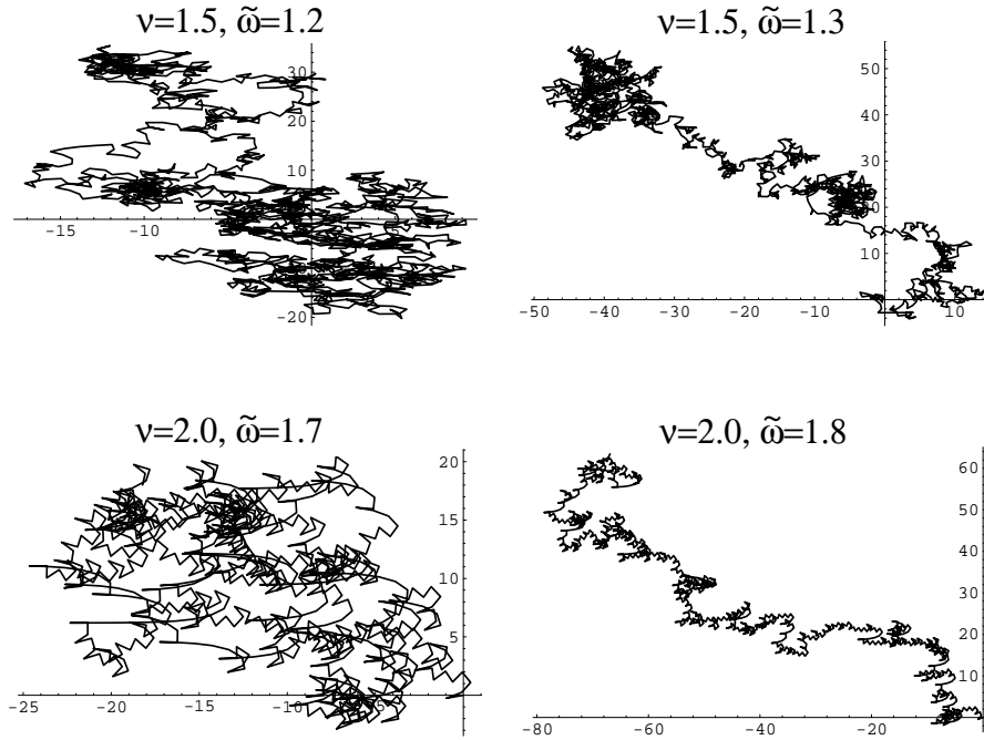
Fig. 2.18. Sample paths of Brownian tip motions due to asymptotically homoclinic shape dynamics.
