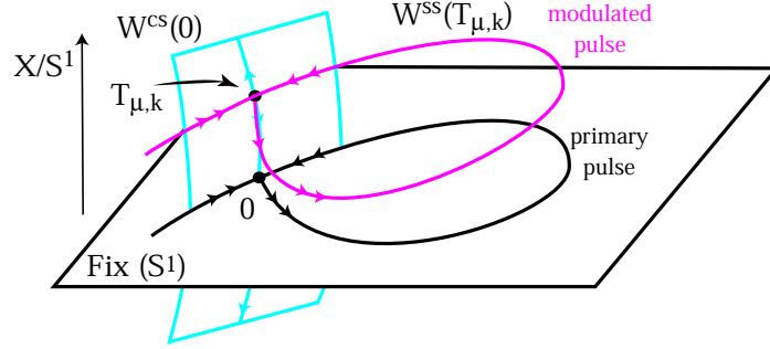
Fig. 2.14. The homoclinic bifurcation creating a modulated pulse travelling through a Turing pattern. See Plate ?? in the Appendix for a version of this figure in colour.
