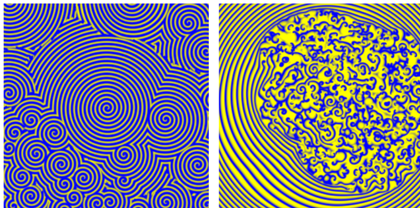
Fig. 2.26. Final state after farfield and core breakup. See Plate ?? in the Appendix for a version of this figure in colour.
