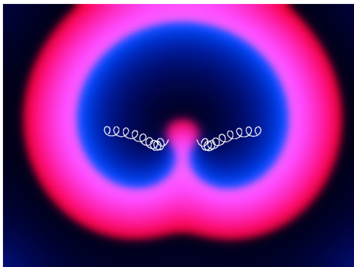
Fig. 2.33. [FiMa00, Fig. 7] Meandering interaction and collision of a pair of planar spiral waves. See Plate ?? in the Appendix for a version of this figure in colour.
