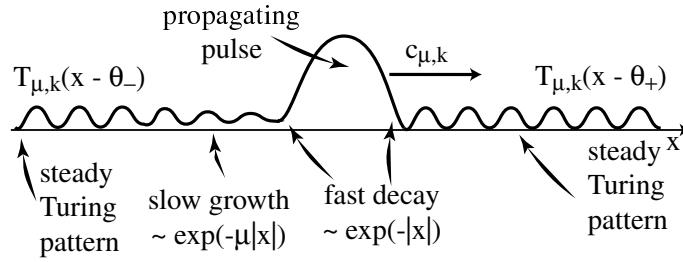
Fig. 2.9. A modulated pulse moving through a Turing pattern
