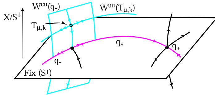
Fig. 2.13. The heteroclinic bifurcation failure of a front leaving a Turing pattern behind. See Plate ?? in the Appendix for a version of this figure in colour.
