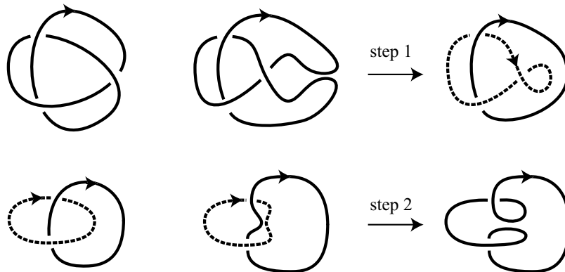
Fig. 2.32. Schematic two-step disintegration of a torus knot filament via linked filaments.
