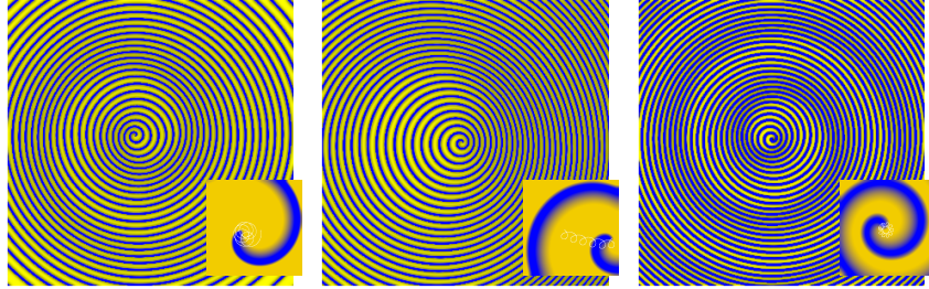
Fig. 2.22. Farfield patterns and tip motion in case of inward meander, drift, and outward meander. The large pictures show the superspiral-shaped deformations of the primary spiral. The small inlets show, on a smaller spatial scale, the tip motion. See Plate ?? in the Appendix for a version of this figure in colour.
