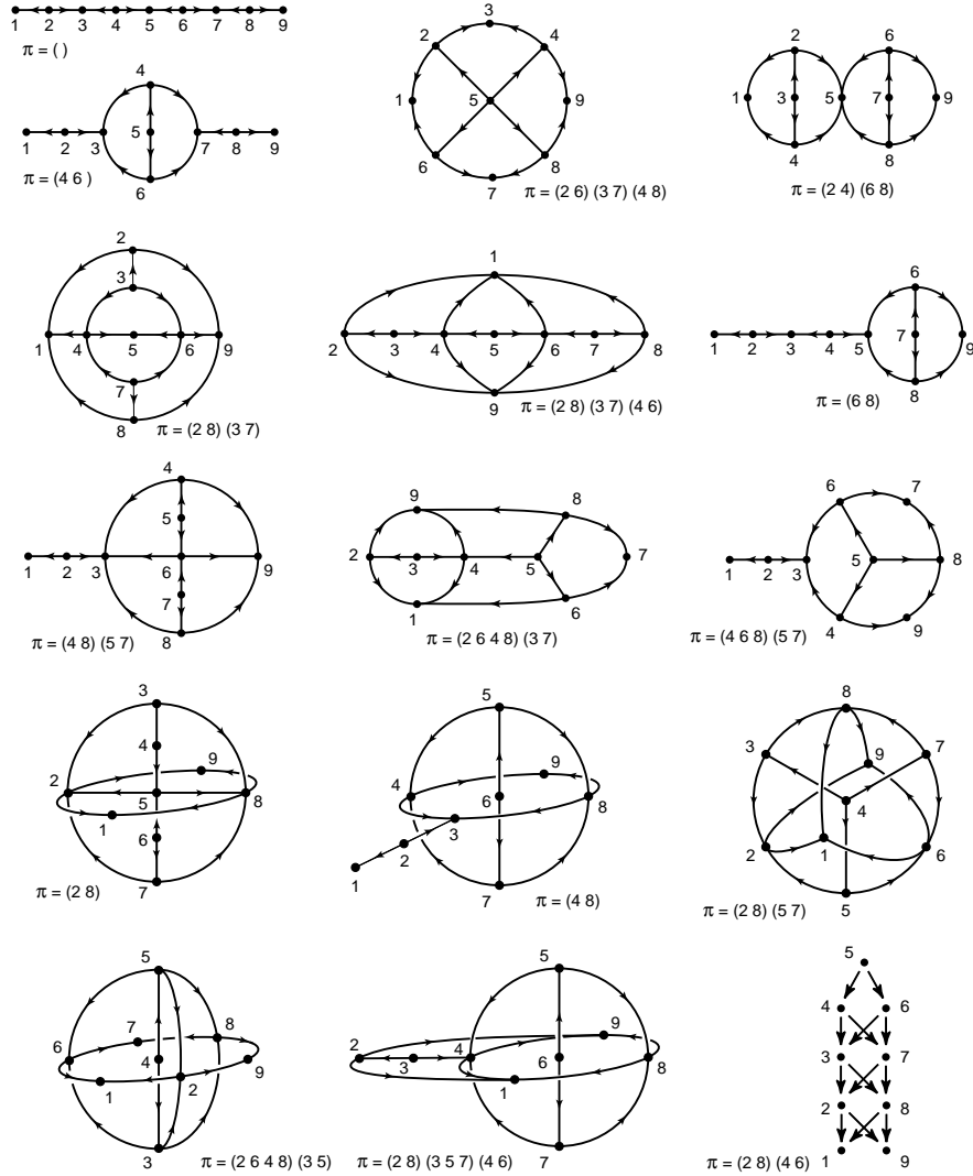
Fig. 2.2. All sixteen Sturm attractors \mathcal{A}_f with n = 9 equilibria. The corresponding Sturm permutations \pi_f are indicated in cycle notation.
