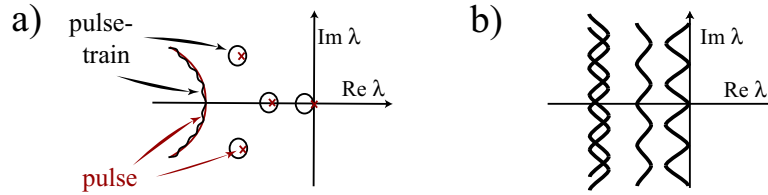
Fig. 2.19. The spectrum of wavetrains of weakly interacting pulses in the steady frame (a), and the Floquet exponents in the comoving frame (b).
