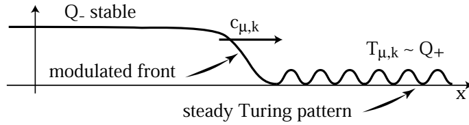
Fig. 2.7. A modulated front invading a Turing pattern, case I
