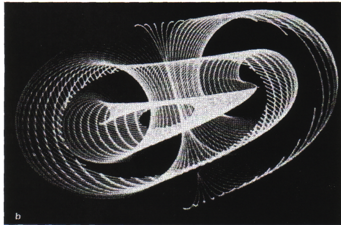
Fig. 2.27. Scroll waves are stacks of spirals (a). Twisted scroll wave (b). Courtesy of [PaWi85].
