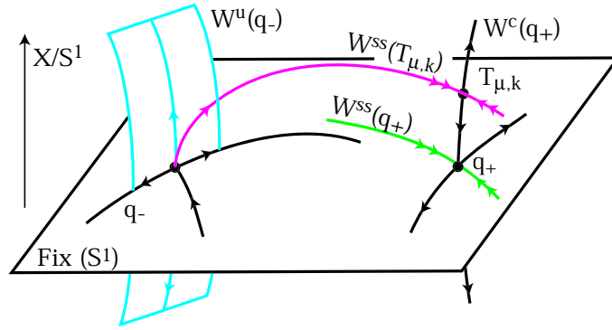
Fig. 2.12. The heteroclinic bifurcation creating a modulated front which invades a Turing pattern. See Plate ?? in the Appendix for a version of this figure in colour.
