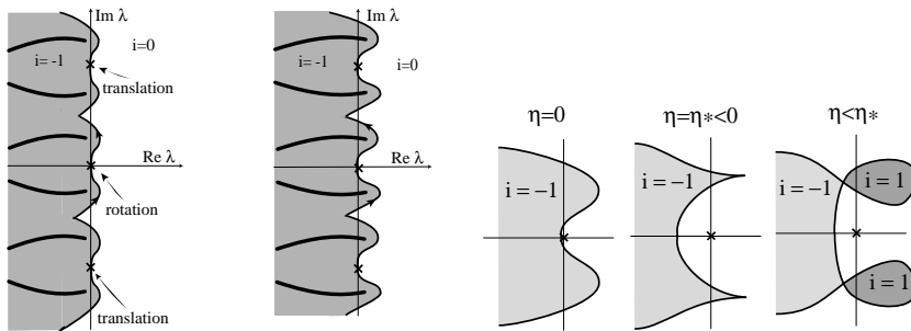
Fig. 2.23. Schematic plot of essential and absolute spectra crossing the axis successively at farfield breakup.
