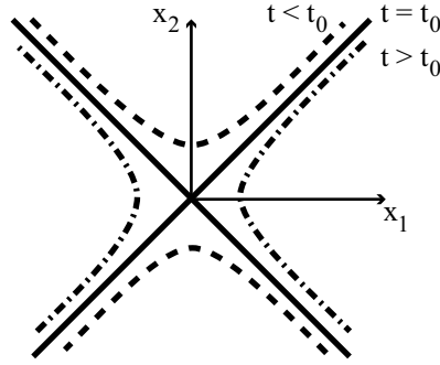
Fig. 2.31. Zero sets of u(t, x) according to (2.229) as t passes through t_0 .
