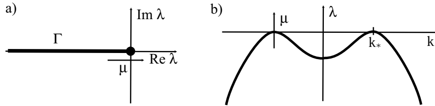
Fig. 2.5. The critical curve \Gamma_+^{\ell} \subset \mathbb{C} , (a) , and the temporal eigenvalue \lambda_+^{\ell} as a function of the wavenumber k , (b) , are shown at criticality.
