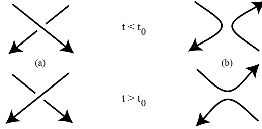
Fig. 2.29. Two scenarios for topology changes of linked scroll filaments: (a) break through; (b) crossover.
