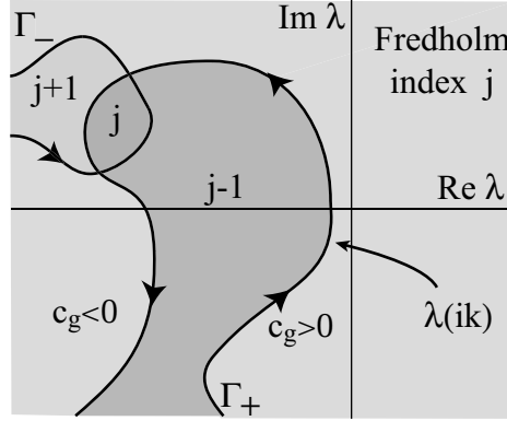
Fig. 2.4. A schematic plot of the oriented spectral curves \Gamma_\pm^\ell and the Fredholm indices of \mathcal{L}_* - \lambda .
