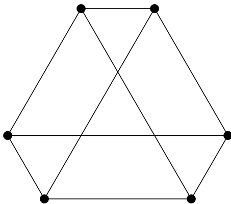
Figure 13. The convex hull of the moment graph of the flag manifold \mathcal{F}\ell_3 is a permutohedron
