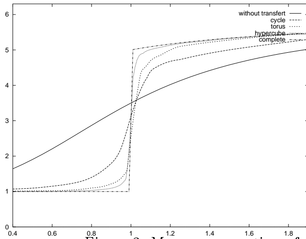
Figure 3: Mean response times for K=6 .
