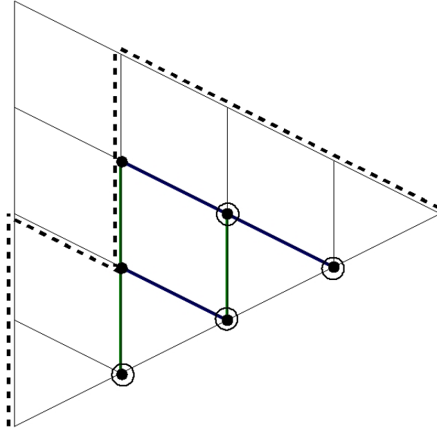
Figure 2.2: A Dyck path (dashed line) overlaid on P_4(\{b, g\}) . The order ideal corresponding to this path consists of all the circled poset elements.
