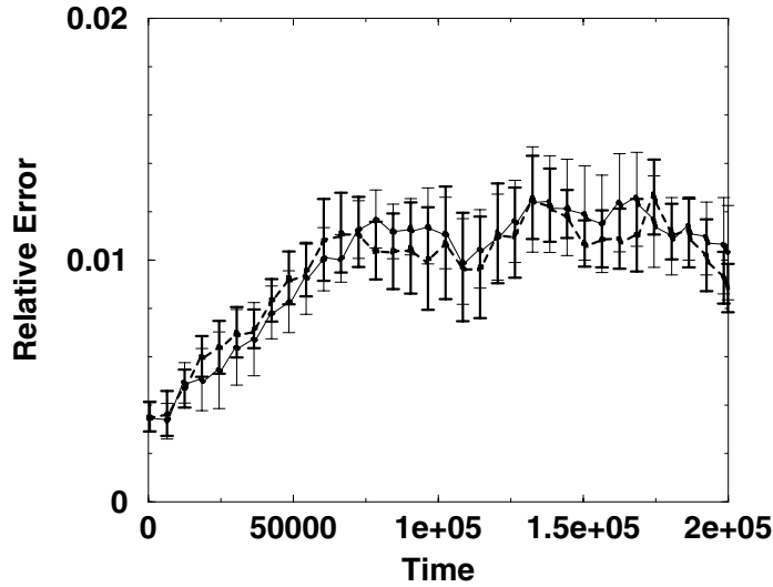
FIG. 12. Comparison of relative errors for CI solutions (using local SVD basis vectors) corresponding to two different flagellar reinitialization schemes. The signal transduction variables were initialized to their local equilibrium values, \bar{u}_j = \{0, f(S(x_j))\} . In one case, all flagella were started in the CW state, shown in the thin solid line; in the second case, all flagella were started in the CCW state, with those cells to the left (right) of the chemoattractant peak running right (left), shown in the thick dashed line. The points correspond to averages over N_{MC} = 5 realizations starting from different random number seeds. The error bars denote the error on the mean, \sigma_{\bar{\epsilon}} .
