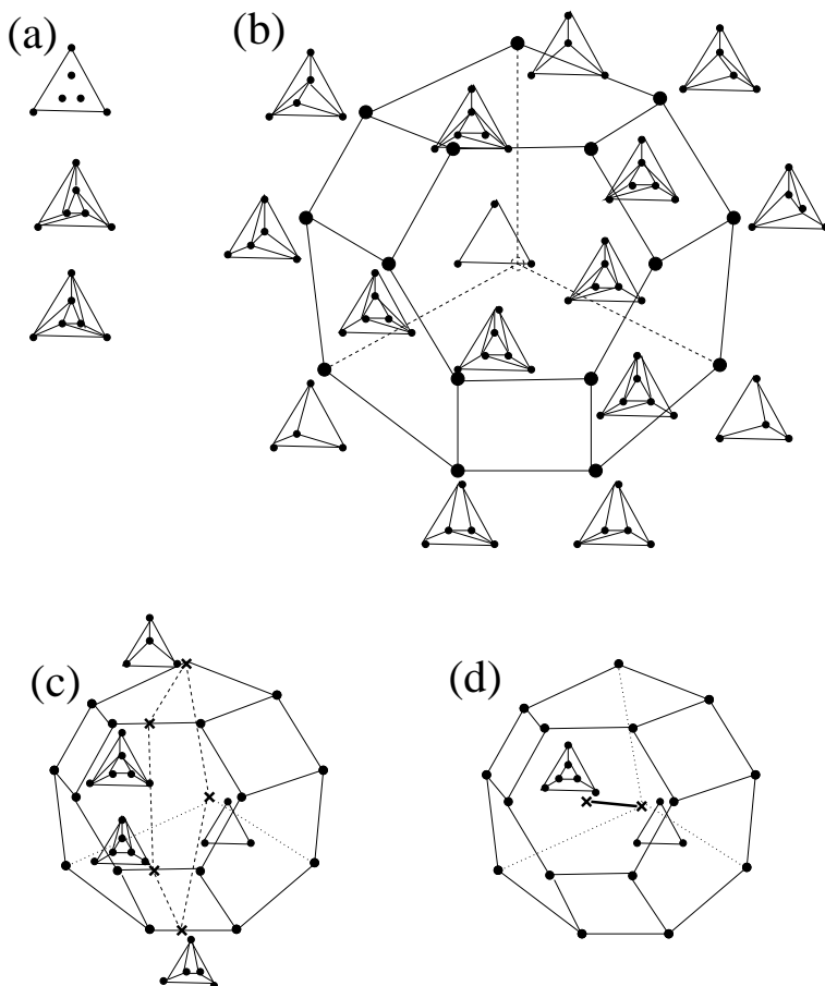
FIGURE 2. Equivariant secondary polytopes for subgroups G of the dihedral group D_6 acting on the point configuration \mathcal{A} shown in (a).
