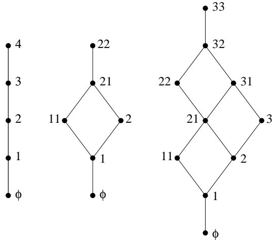
Figure 6.1: The lattices L(1, 4) , L(2, 2) , and L(2, 3)
