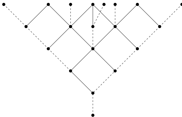
Figure 8.1: The poset Z up to level five
