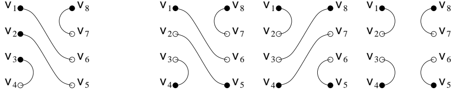
FIGURE 4.2. A one-element subset of T_4(2) corresponding to \Delta_{123,234}(x)\Delta_{4,1}(x) and a three-element subset of T_4(2) corresponding to \Delta_{14,23}(x)\Delta_{23,14}(x) .
